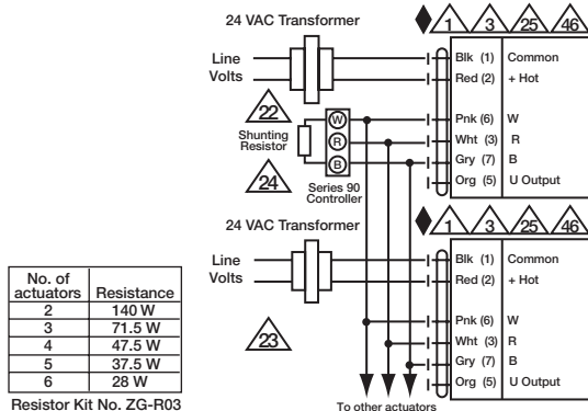
Multiple Actuators
