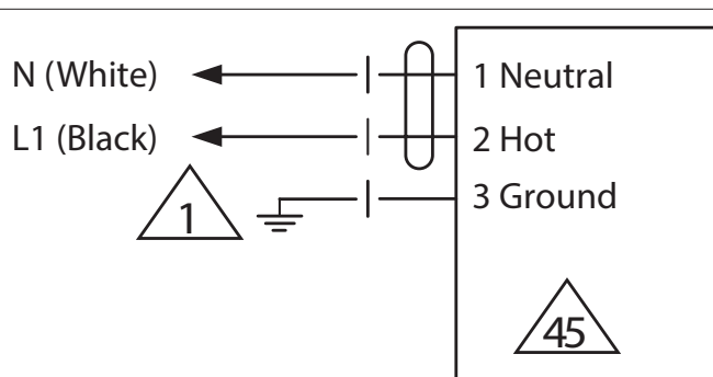
120 VAC
