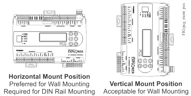
Figure 1: FX-PCG2621 Mounting Positions
