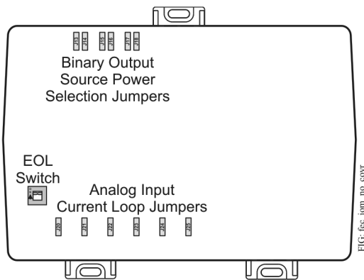
Figure 10: FX-PCG26 with Cover Removed Showing EOL Switch and Jumper Positions
