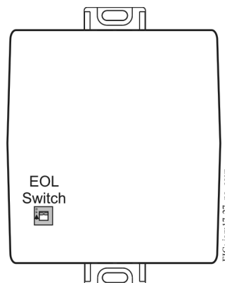
Figure 11: FX-PCX17 or FX-PCX27 with Cover Removed Showing EOL Switch Location
