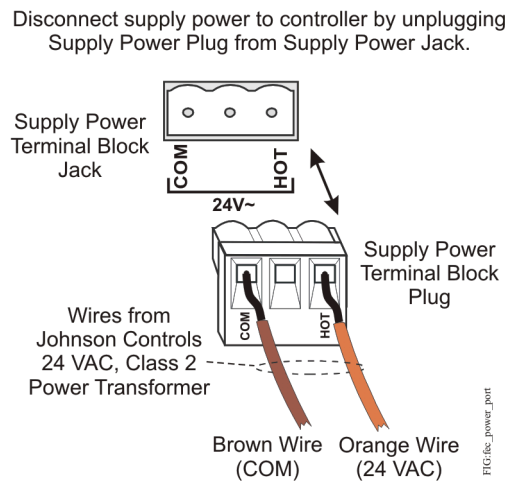
Figure 8: 24 VAC Supply Power Terminal Block Wiring
