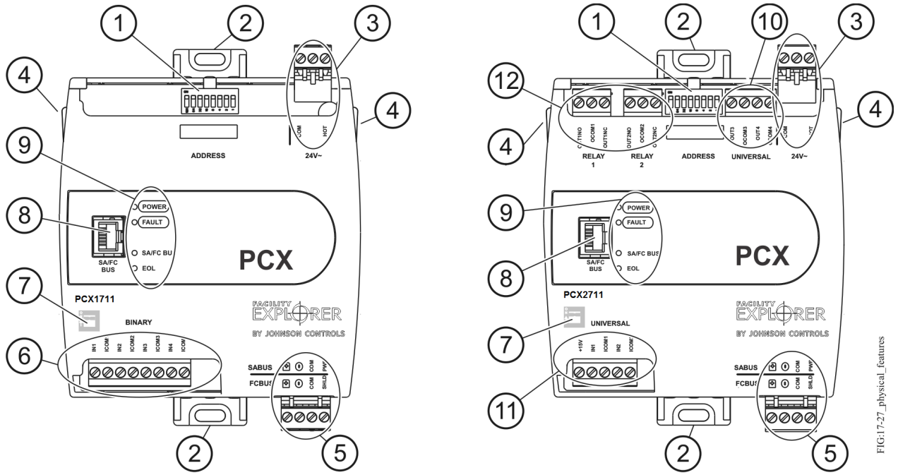
Figure 3: FX-PCX17 and FX-PCX27 Physical Features
