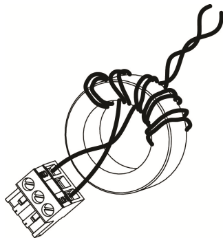
Figure 7: Wrapped Ferrite Ring
