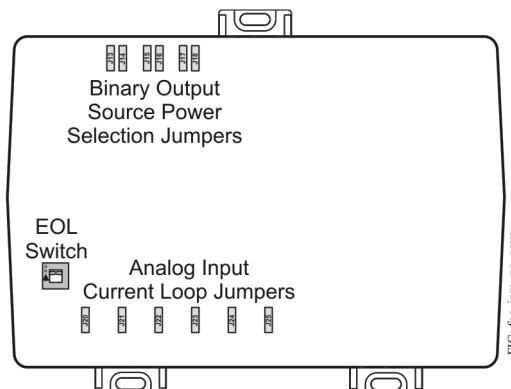
Figure 10: FX-PCX47 with Cover Removed Showing EOL Switch and Jumper Positions
