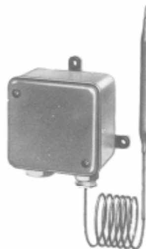
Fig. 2: Control with NEMA 3R rainproof enclosure.
