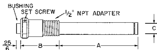
Fig. 3 — Bulb Well for liquid immersion applications where temperature bulb may be removed without draining tank.
