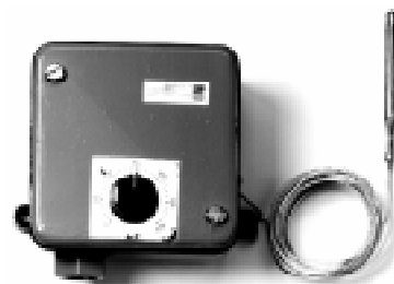
Fig. 1: Industrial control with remote bulb, NEMA 4 watertight enclosure.
