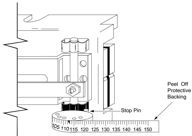
Figure 5: Applying Dial Strip to Setpoint Dial
