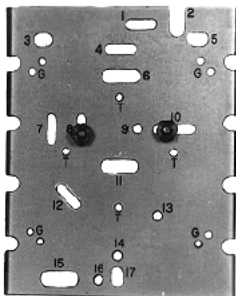
Subplate for Later Style Wallbox and Mortar Joint
