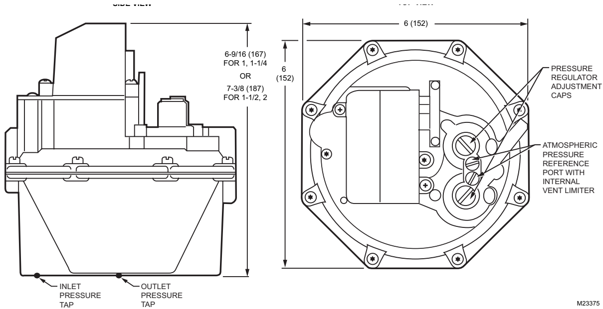
Fig. 1. V4943/44 and V8943/44 dimensions in in. (mm).
