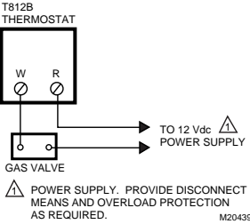
Fig. 6. T812B in 12 Vdc application.
