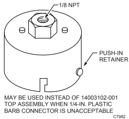
Fig. 4. 14003648-001 Vandalism Shield.
