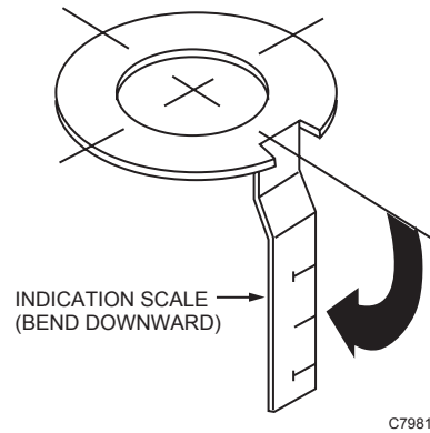
Fig. 3. 14001101-001 Position Indicator.
