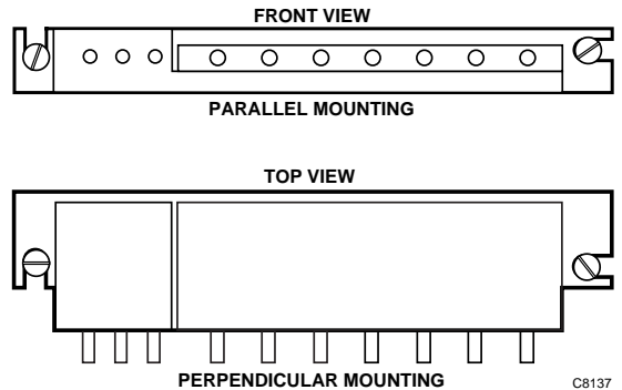
Fig. 3. Parallel and Perpendicular Mounting.
