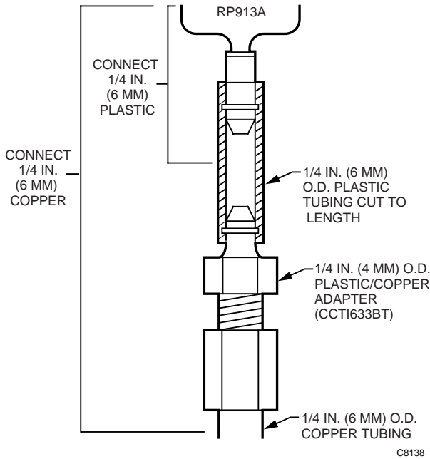
Fig. 4. Adaptation Piping.
