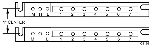
Fig. 2. Dimensions for Two RP913As.
