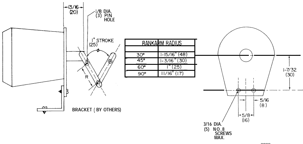
Fig. 2. Bearingless Application with a Pinned Shaft (90 Degrees Maximum).
