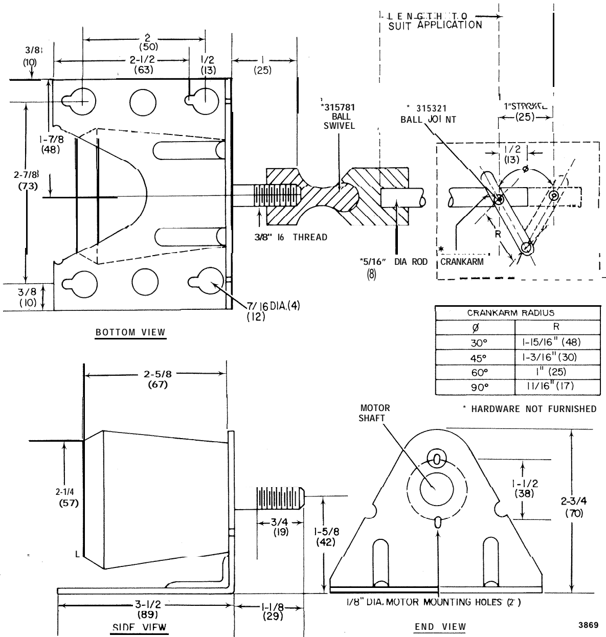
Fig. 3. Typical Crankarm Application Using Part No. 14003 640-00 1 Mounting Bracket.
