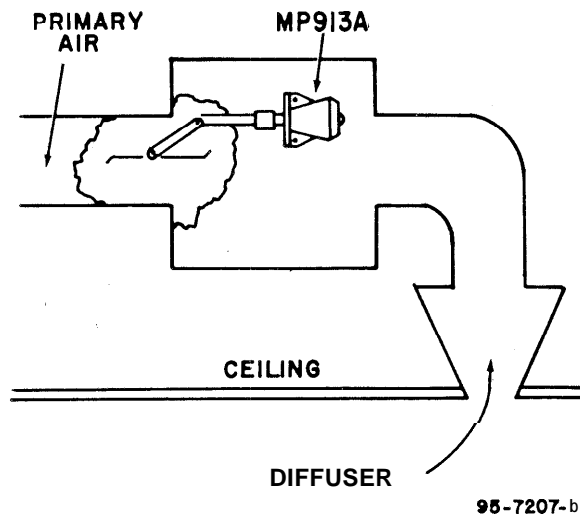
Fig. 1. Mounting in Variable Volume Mixing Box.
