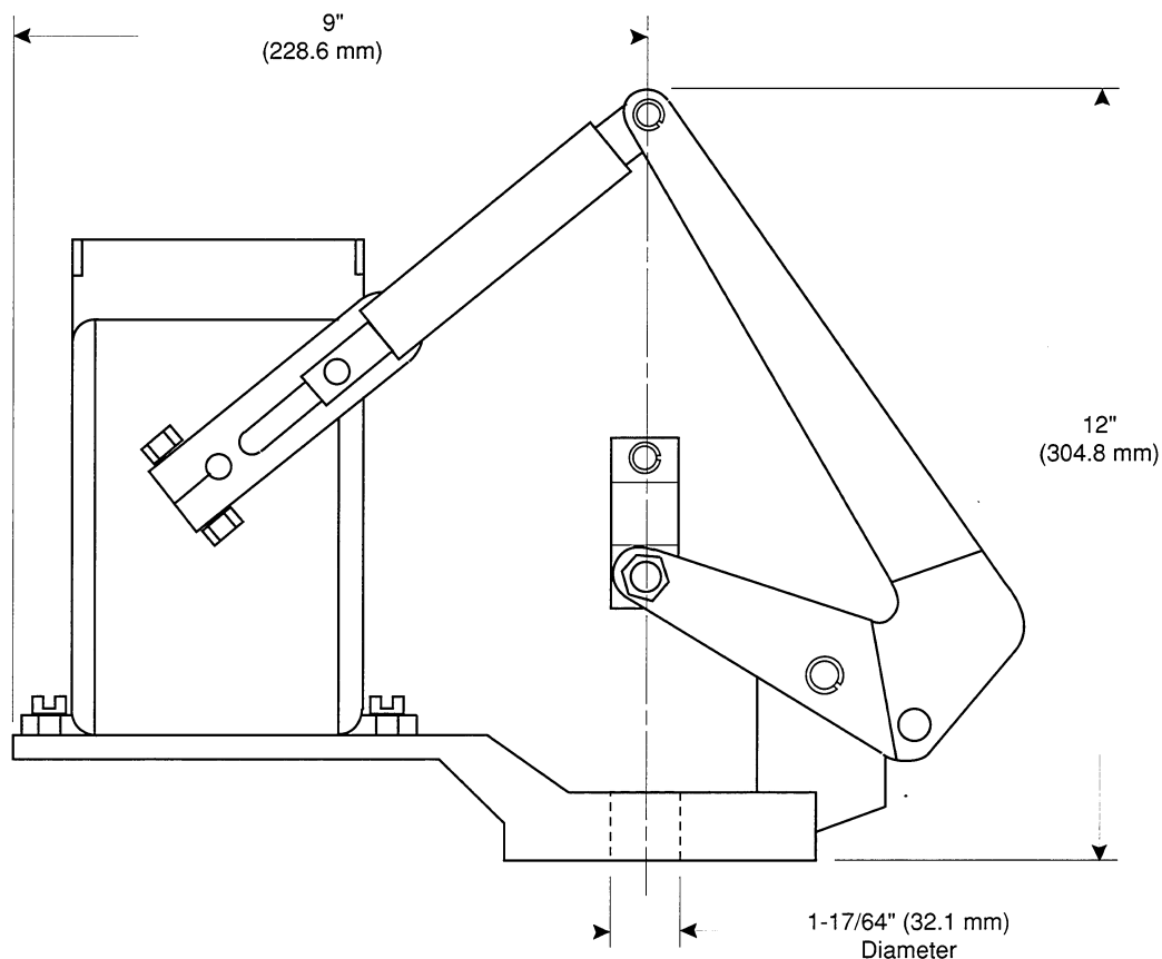
Figure-3 Mounting Dimensions of Valve Linkage Assembly.
