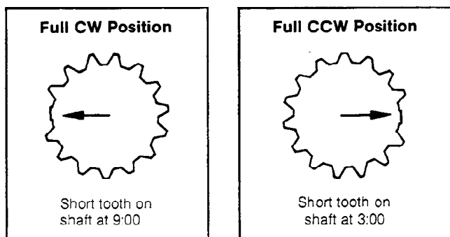
Figure 2. Actuator Shaft Position (Front View)
