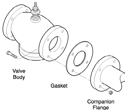
Figure-5 Installation of Flanged End Valves.
