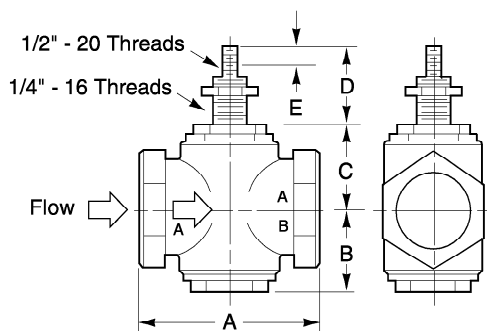
Figure-6 Typical of VB-9223-0-4-P, 2-1/2" and 3" Valve Bodies.
