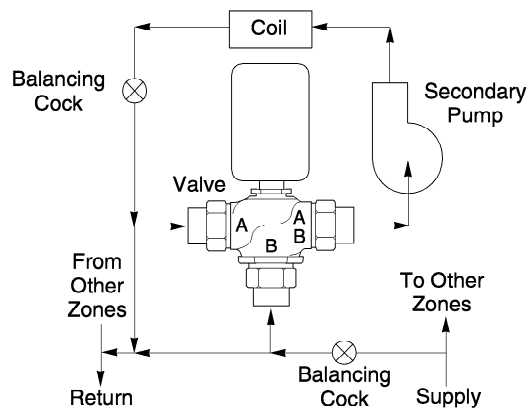
Figure-5 Typical Primary-Secondary Piping.
