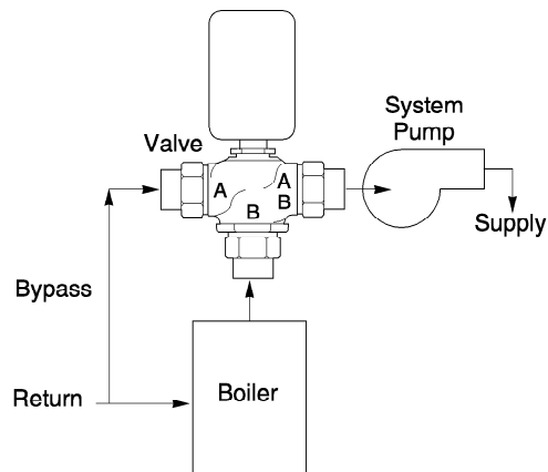
Figure-4 Typical Boiler Piping When Used in a Hot Water Reset Application.
