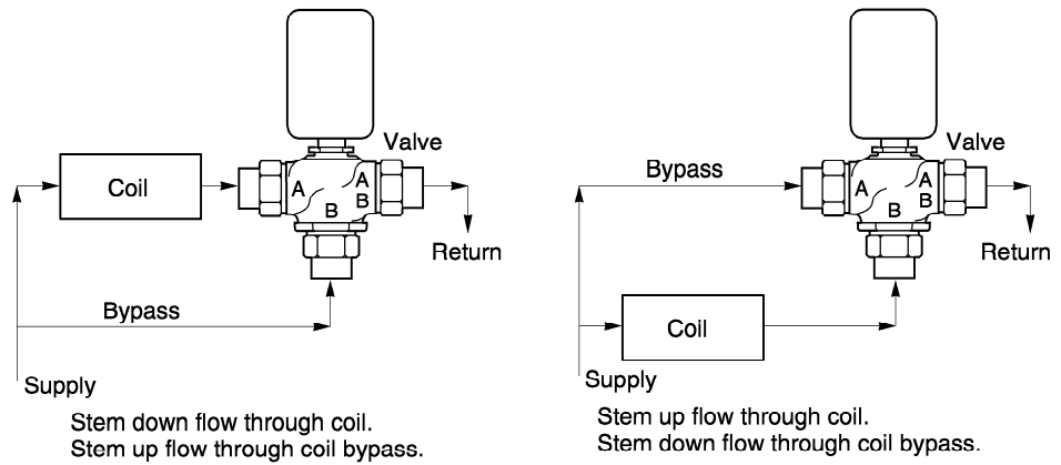
Figure-3 Typical Piping for Control of Heating or Cooling Coil.
