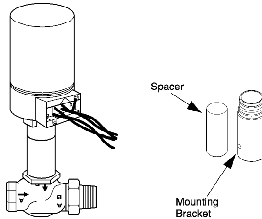
Figure-1 Installation of AV-601.
