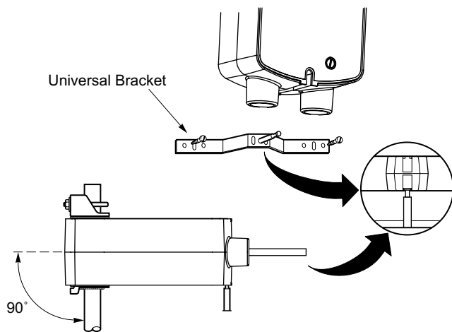
Figure-7 Mounting Universal Bracket to Actuator.
