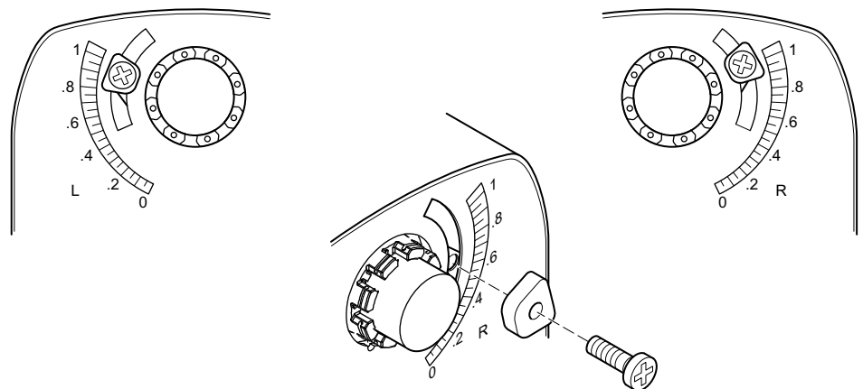
Figure-11 Adjusting Stop Block for Limited Rotation.
