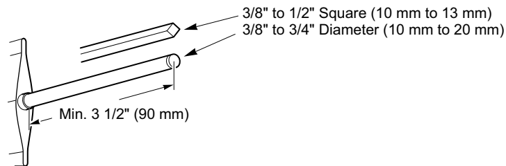
Figure-4 Long Damper Shaft Dimensions.
