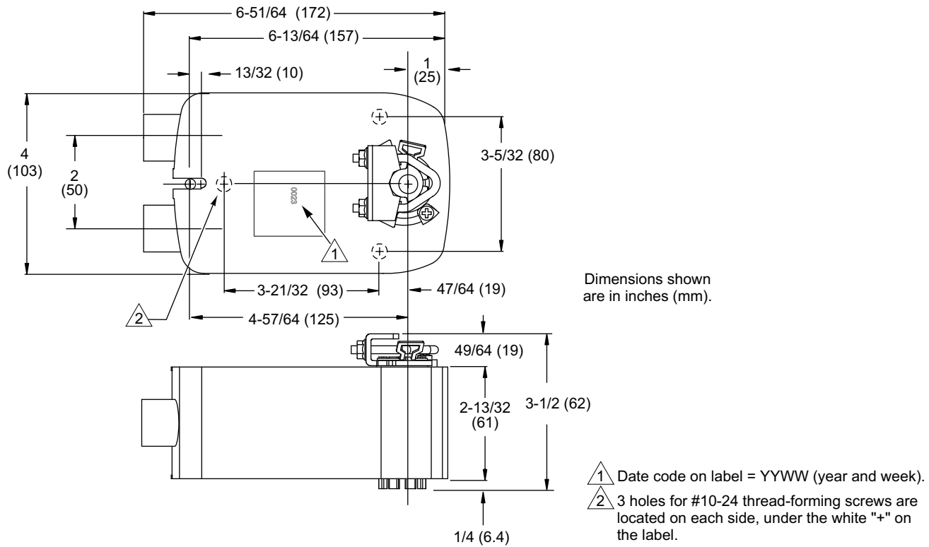
Figure-12 MX40-704X Series Mounting Dimensions.
