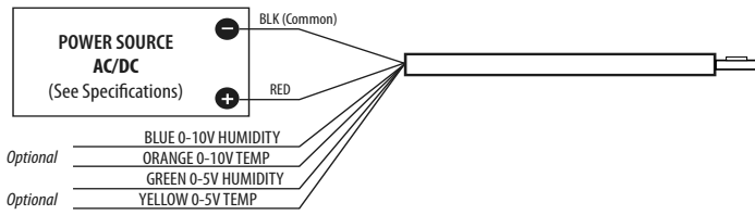
HO Series Outside Air (0–5V/0–10V Temperature Transmitter Versions)
