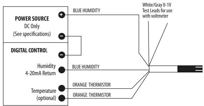
HO Series Outside Air (4-20mA Resistance Versions)
