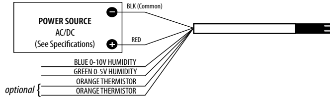
HO Series Outside Air (0–5V/0–10V Resistance Versions)
