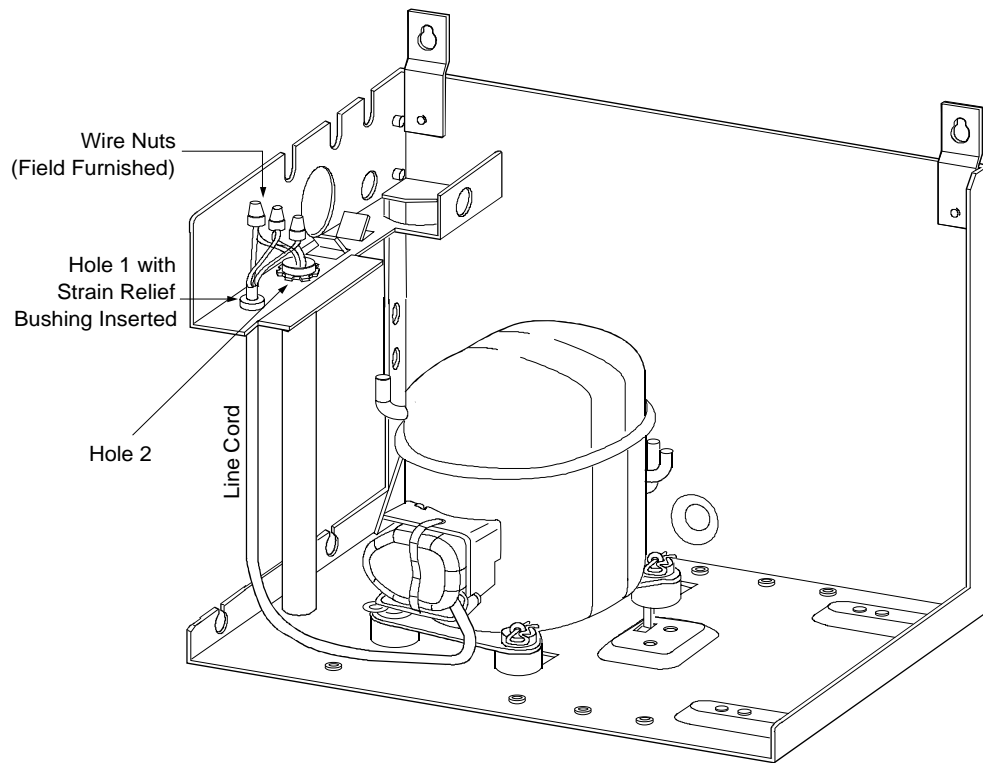
Figure 3: Permanent Wiring Using Conduit
