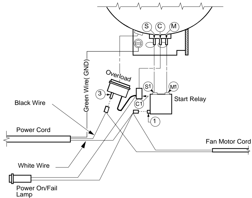
Figure 13: Air Dryer Compressor Motor Wiring Diagram
