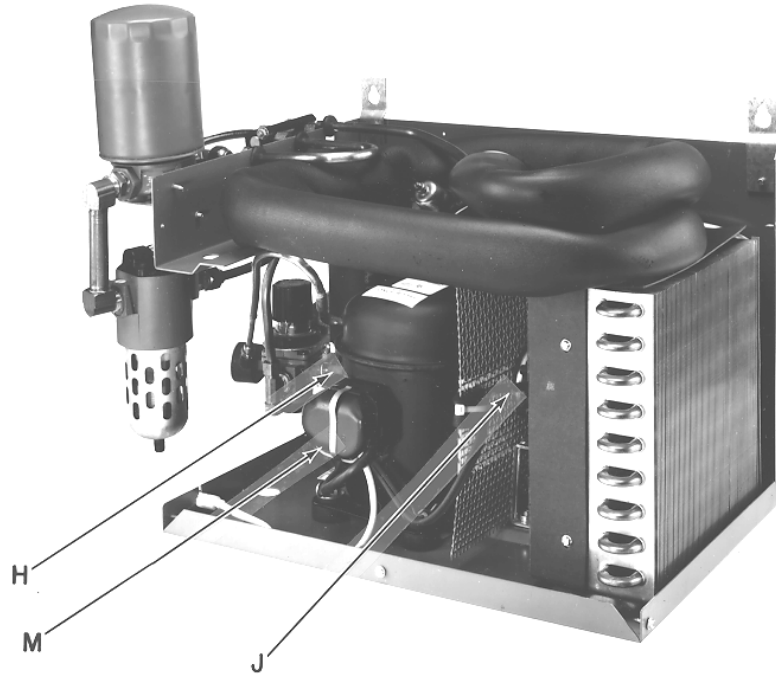
Figure 14: Repair Parts (See Table 3)
