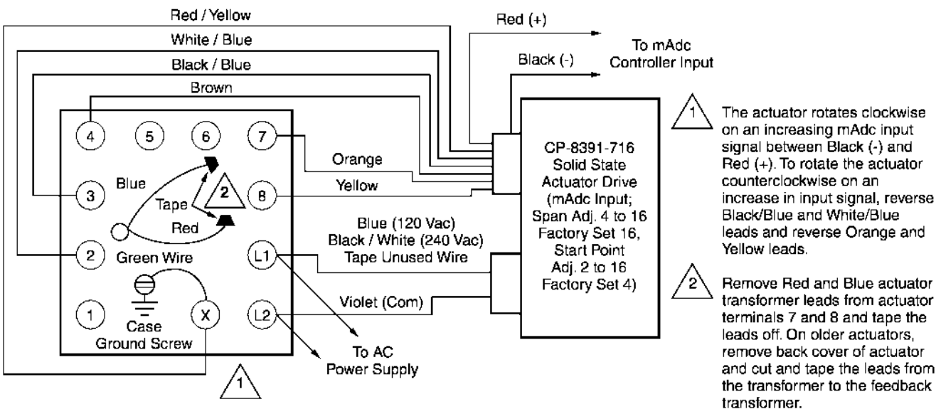
Figure-23 External Wiring for CP-8391-716, mAdc Interface with Line Voltage Actuators with Internal Transformer.
