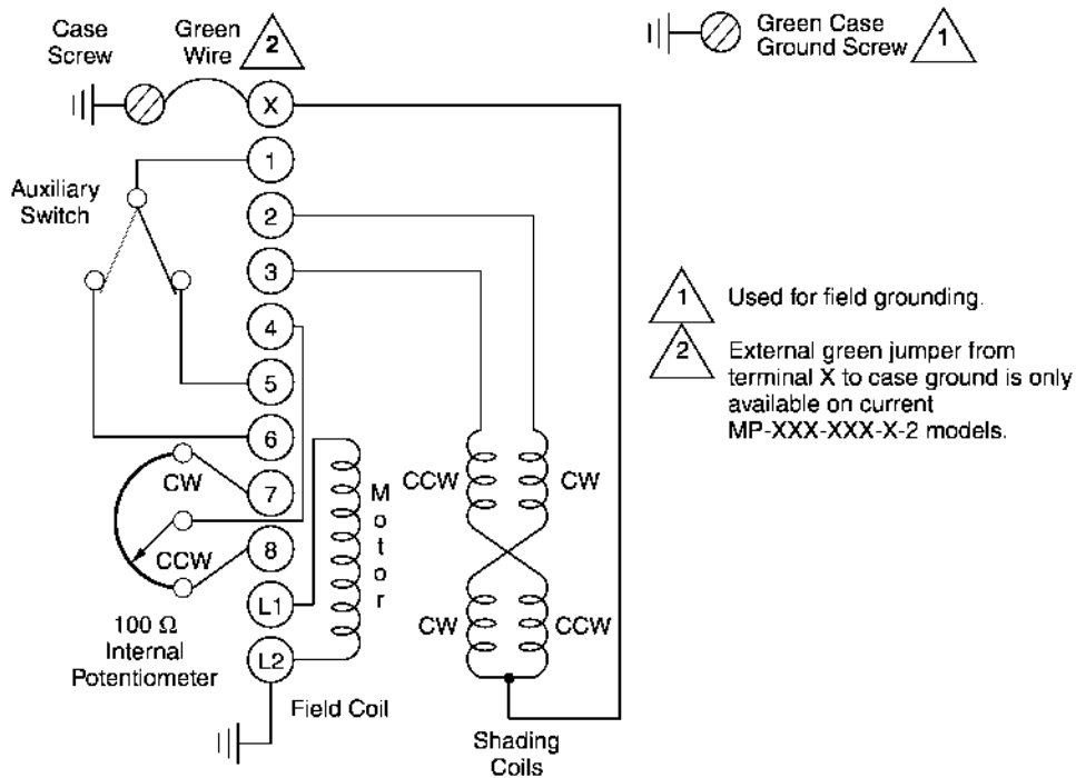
Figure-28 Internal Wiring for Line Voltage Actuators without Limit Switches (Actuator is Stall Type with Built-in Mechanical Stops.)
