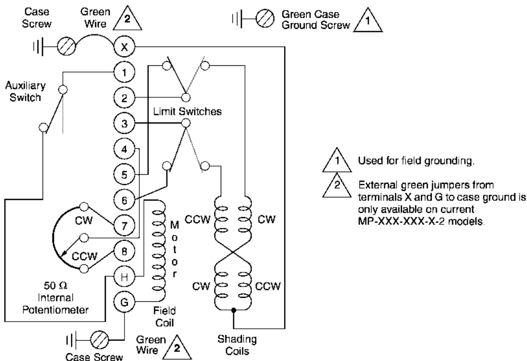
Figure-32 Internal Wiring for 24 Vac Sequencing Actuators.
