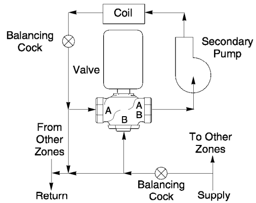
Figure-7 Typical Primary-Secondary Piping.
