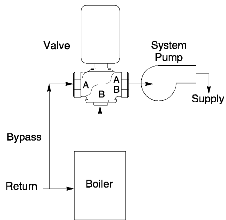
Figure-6 Typical Boiler Hot Water Reset.
