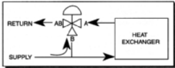
Figure 4 Three-Way Valve Piping.
