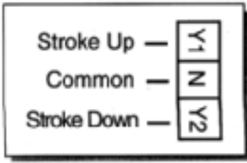
Figure 3 VAT340 Non-Spring Return.
