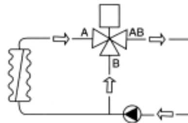
Figure 3 Three-Way Flow Direction.
