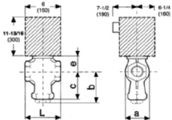
Figure 5 Dimensions.
